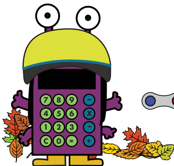
Cal Culculator
